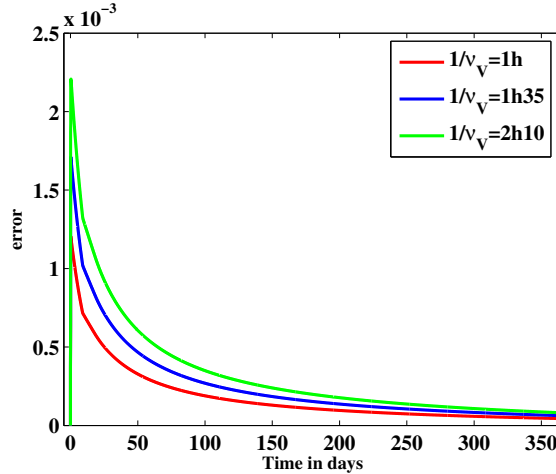
Figure 3: Error between the full and the reduced system for the same non zero initial data and different \nu_V . Precisely \text{error}(t) = |x^\epsilon(t) - x(t)| , the parameters \nu, \mu, \alpha, \beta are computed using the relation (2.2) with the approximation P_C^0 = P_C for the parameter value of the Table 1. The initial data for y is y_0 = 0.5 and the initial data for x and x^\epsilon is \varphi(t) = 0.6 for t \in [-9.86, 0] .
