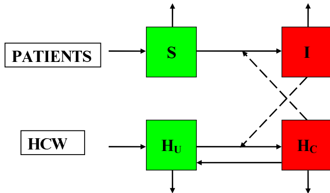
Figure 1: The figure represents a diagram of the individuals fluxes used to describe hospital acquired infections. In this diagram each solid arrow represents a flux of individuals, while the dashed arrows represent the influence of either infected patients or colonized HCWs on the pathogen acquisition.
