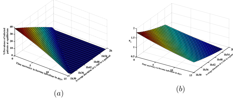
Figure 2: Figures (a) and (b) describe respectively the evolution of the prevalence of infected patients at the equilibrium and R_0 with respect to 1/\nu_V and \tau .
